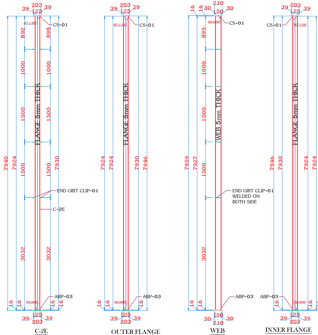
COLUMN DETAIL C-2E @ GRID 1 & 5 QTY:(02,L)(02,R)
